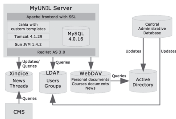
ARCHITECTURE SERVEURS [5]
